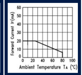
DERATING CURVE
